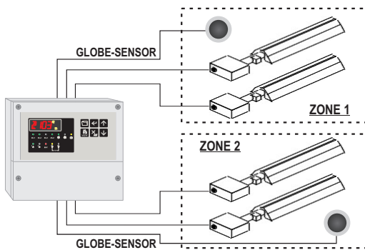
MODO 3: 2 ZONE TERMICHE - 2+2 BRUCIATORI MONOSTADIO MODE 3: 2 THERMAL ZONES - 2+2 SINGLE FLAME BURNERS
