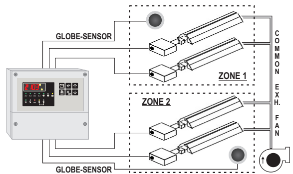
MODO 4: 2 ZONE TERMICHE - 2+2 BRUC. MONOSTADIO + 1 COMM. FAN MODE 4: 2 TH. ZONES - 2+2 SINGLE FLAME BURNERS + 1 COMM. FAN
