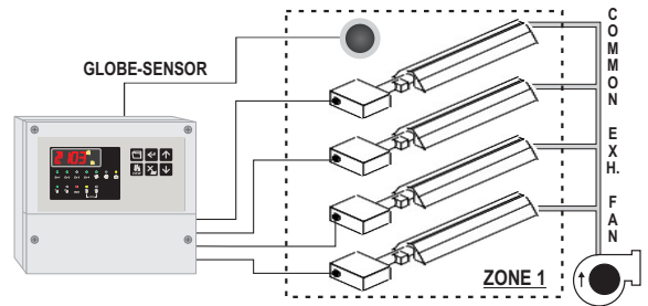
MODO 2: 1 ZONA TERMICA - 4 BRUCIATORI MONOSTADIO + 1 COMM. FAN MODE 2: 1 THERMAL ZONE - 4 SINGLE FLAME BURNERS + 1 COMMON FAN
