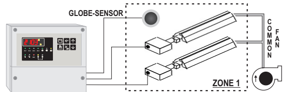
MODO 6: 1 ZONA TERMICA - 2 BRUCIATORI MONOSTADIO + 1 COMM. FAN MODE 6: 1 THERMAL ZONE - 2 SINGLE FLAME BURNERS + 1 COMM. FAN
