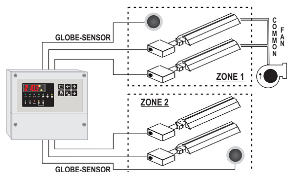
MODO 10: 2 ZONE TERMICHE - ZT 1: 2 BRUC. MONOST. + 1 C.F. // ZT 2: 2 BRUC. MONOSTADIO MODE 10: 2 TH. ZONES - TZ 1: 2 SINGLE FLAME BRNs + 1 C.F. // TZ 2: 2 SINGLE FLAME BRNs
