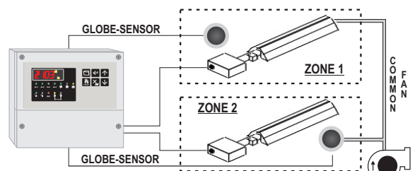
MODO 8: 2 ZONE TERMICHE - 1+1 BRUC. BISTADIO + 1 COMM. FAN MODE 8: 2 TH. ZONES - 1+1 TWO FLAME BURNERS + 1 COMM. FAN
